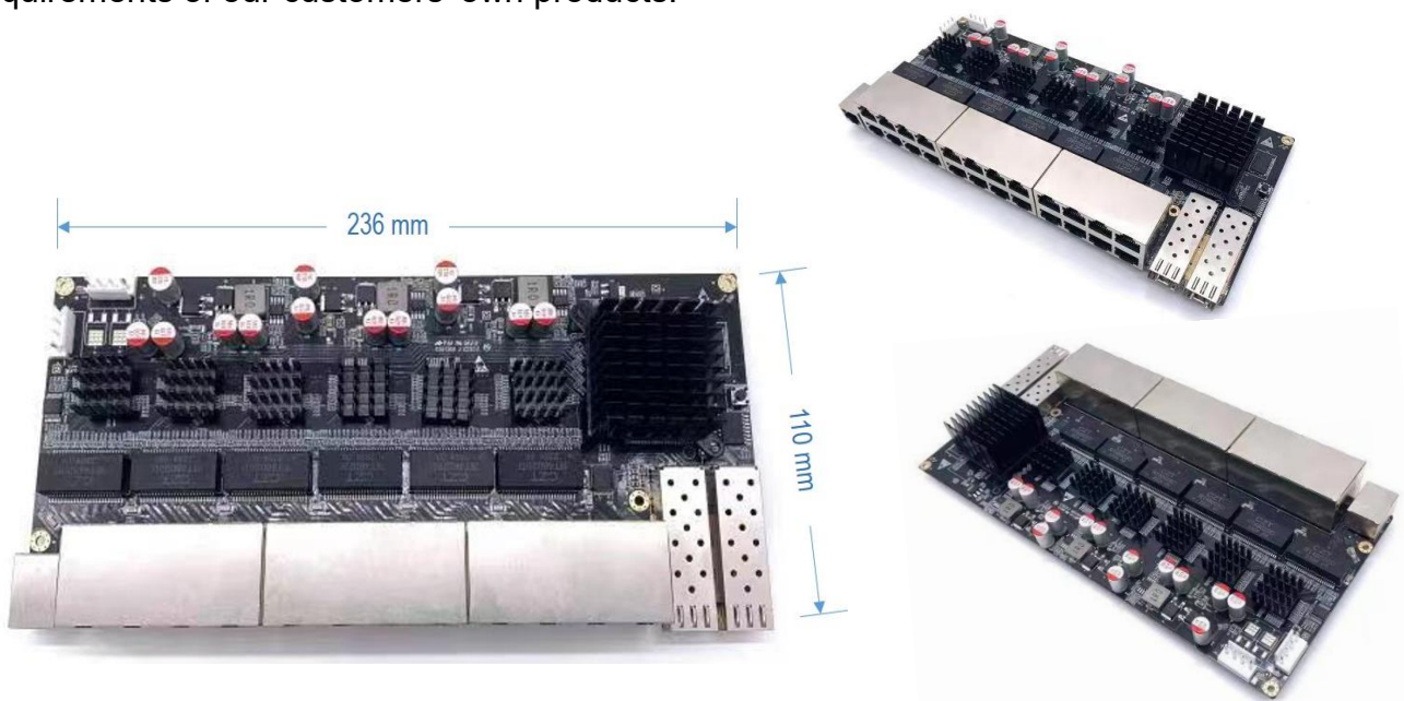
PCBA of the MSQ9224 24x 2.5GT Switch
