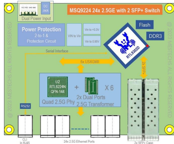
Figure 1. MSQ9224, Block Diagram
